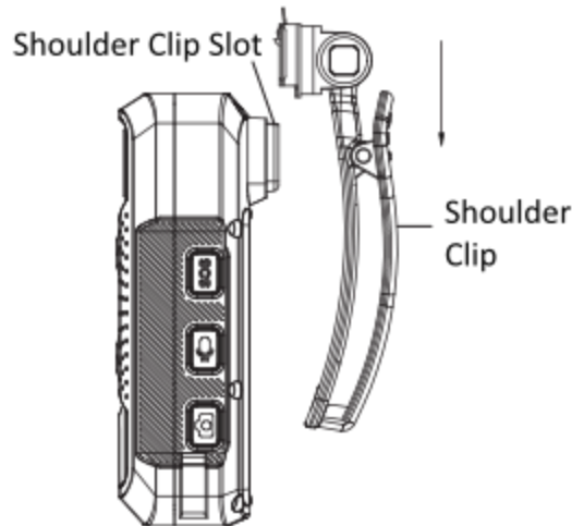
Figure 2-1 Install Shoulder Clip
