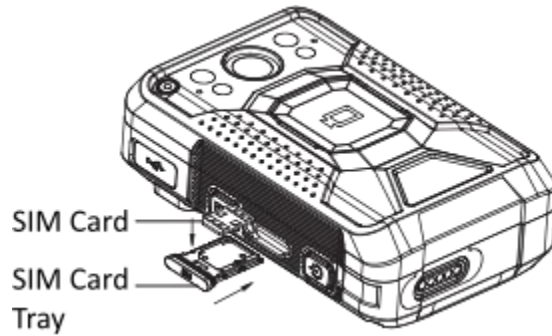
Figure 1-1 Install SIM Card
