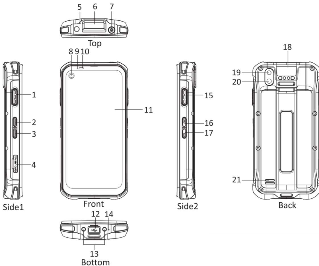
Figure 1-1 Device Overview
