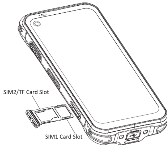
Figure 2-1 Install SIM/TF Card
